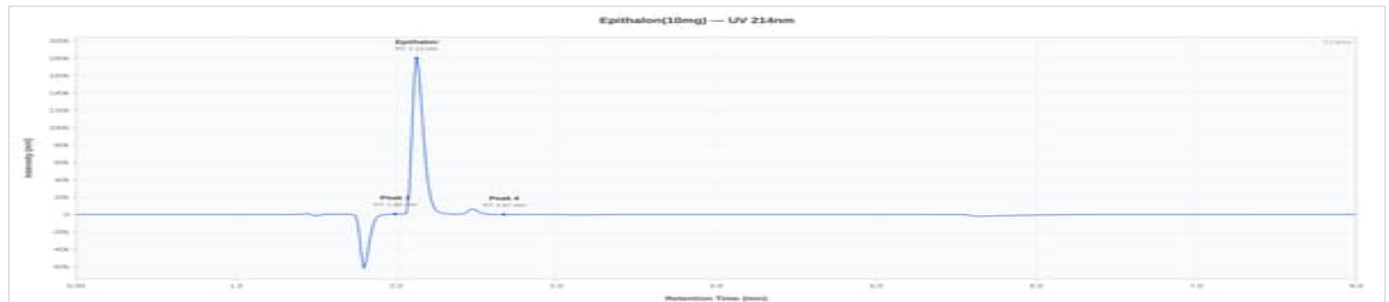
Epithalon 10mg - EP10-101: UV Chromatogram
