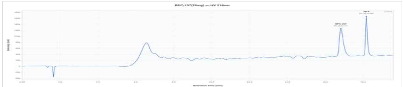
BPC-157 / TB-500 20mg - BB20-101: UV Chromatogram
