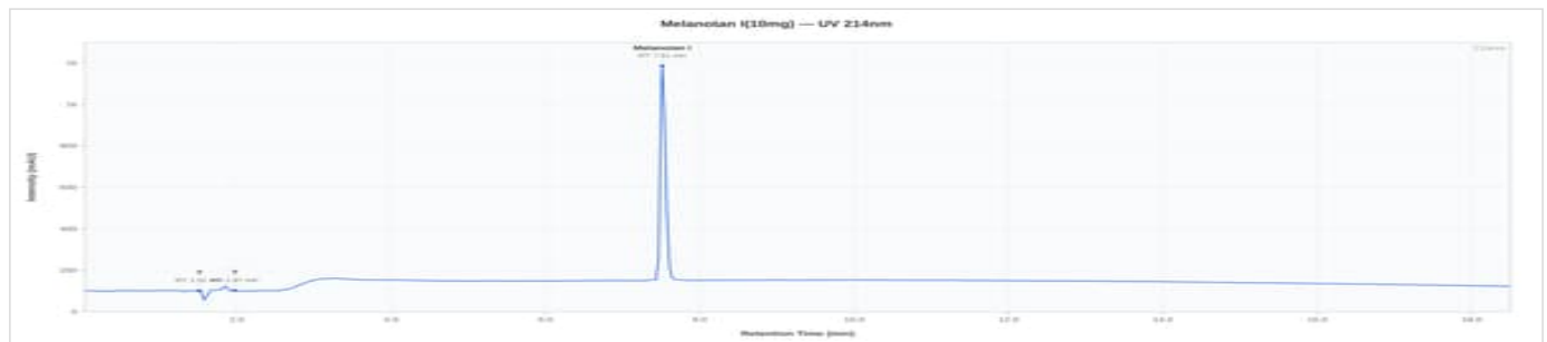
Melanotan I 10mg - MT1-101: UV Chromatogram
