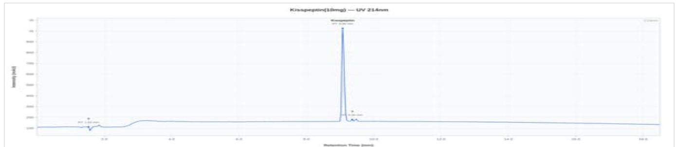
Kisspeptin 10mg - KISS-101: UV Chromatogram
