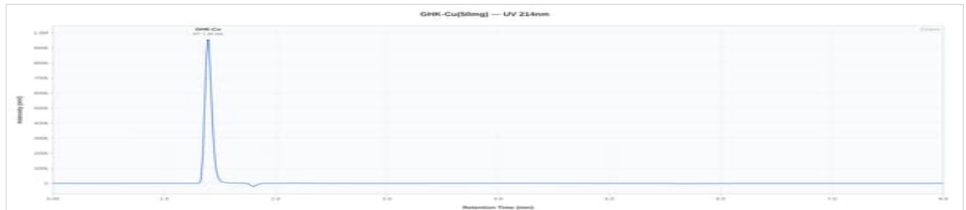
GHK-Cu 50mg - GHK50-101: UV Chromatogram
